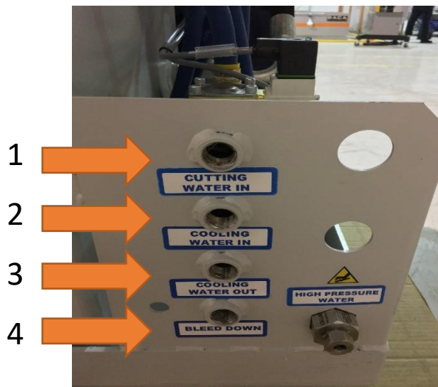
Figure 3 Water Connections
