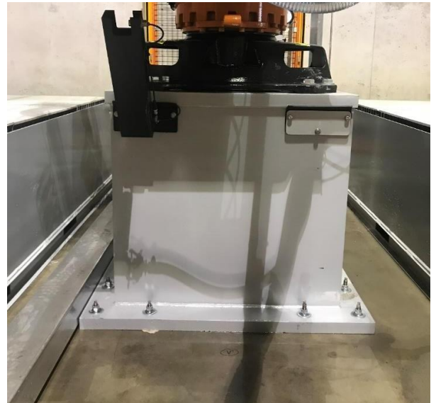
Figure 7: Robot Base Secured to Customer
