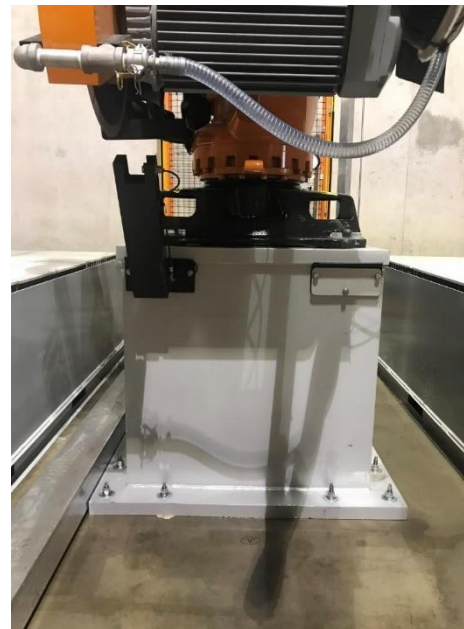
Installed Robo Sawjet pedestal on concrete base
