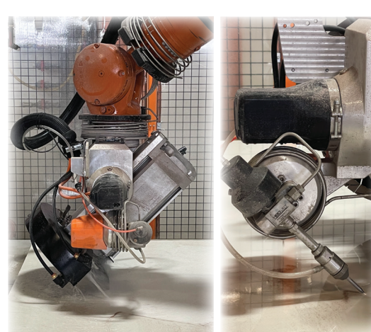
SAW BLADE & JET MITER TOTAL PROCESS CAPABILITY
